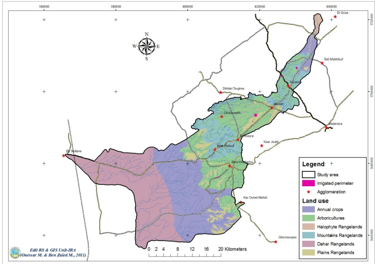
Figure 9: Simplified land use map (adapted from Ouessar, 2007).
