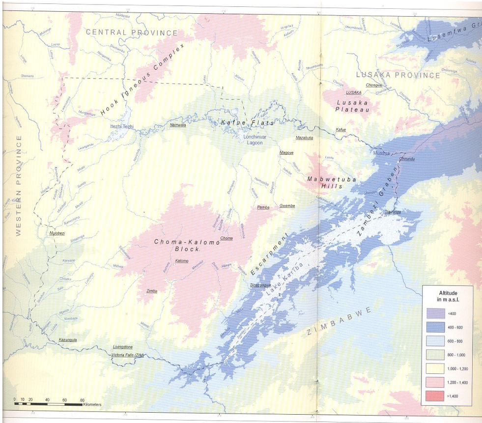
Figure 2: Digital Elevation Model (DEM) with elevation zones at 200 m-intervals.
