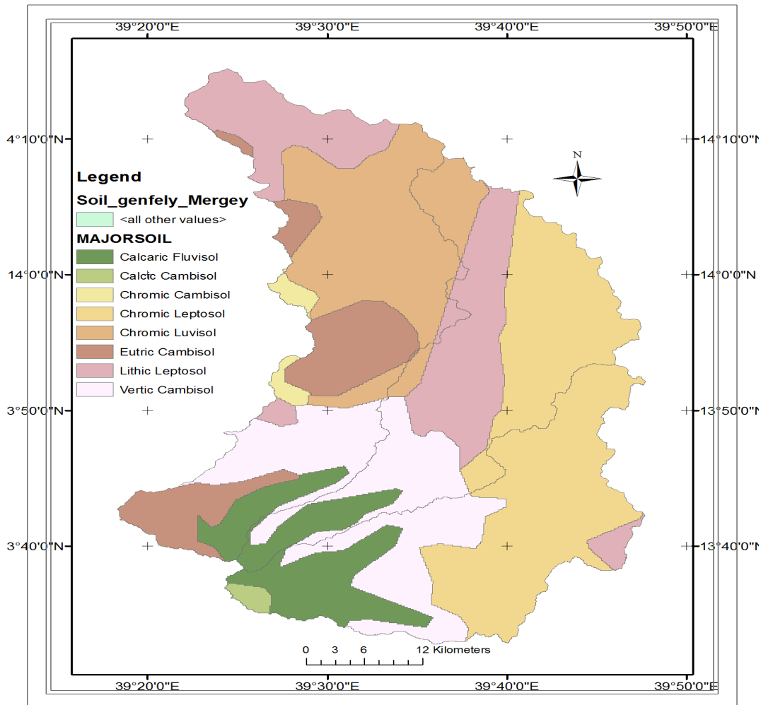
Figure 5 Major soils of the project area (Produced based on Geomorphology and Soils of Ethiopia, Scale 1:1,000,000 (UNDP, FAO, MOA, 1984).
